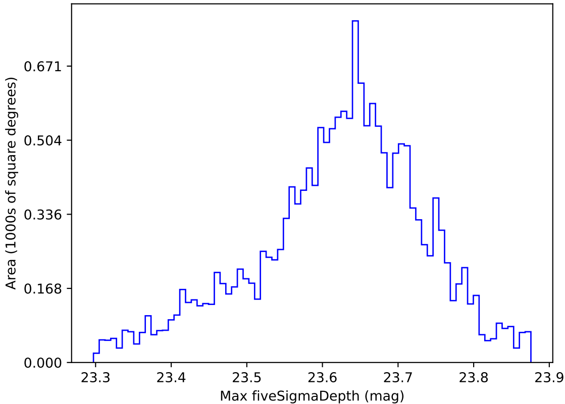
roll_pause_mjdp365_v3.4_10yrs WFD z band: Max fiveSigmaDepth
