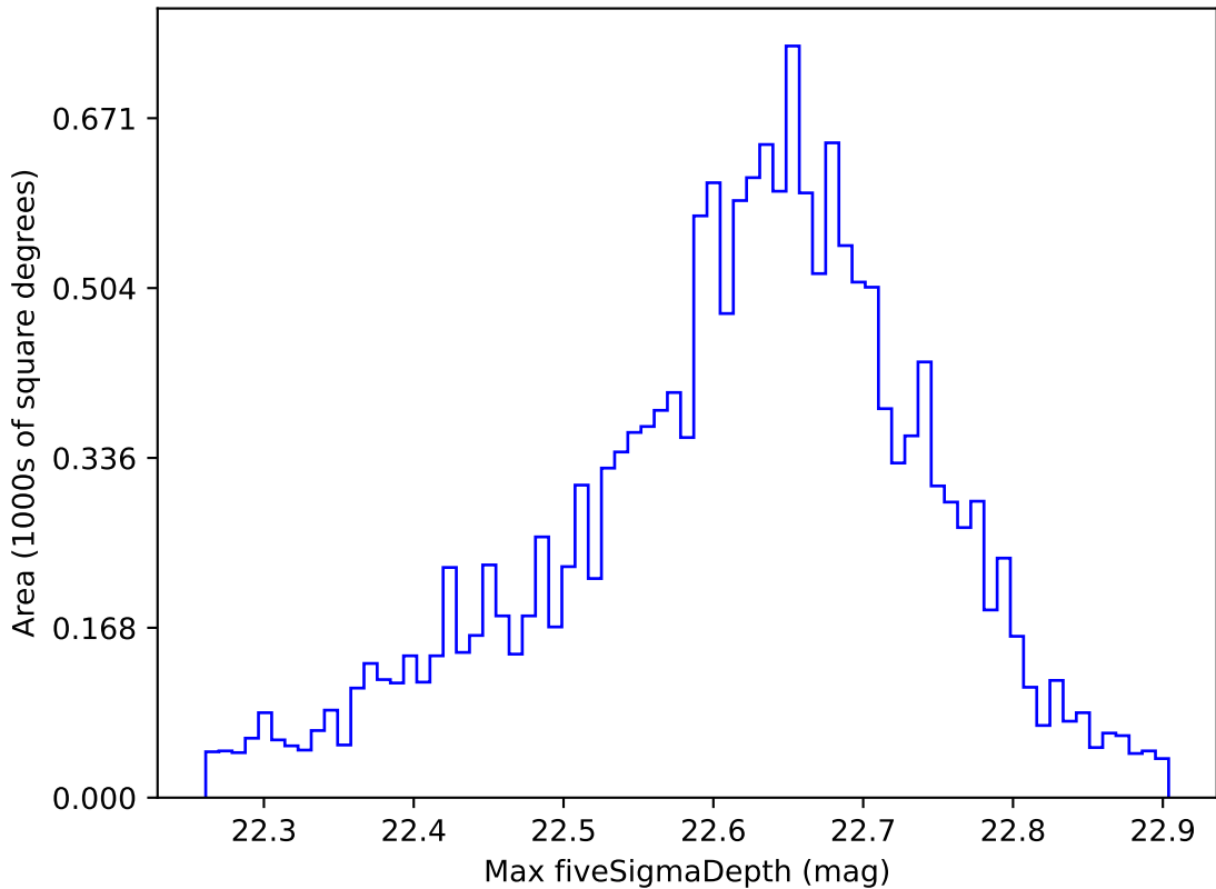
roll_pause_mjdp365_v3.4_10yrs WFD y band: Max fiveSigmaDepth
