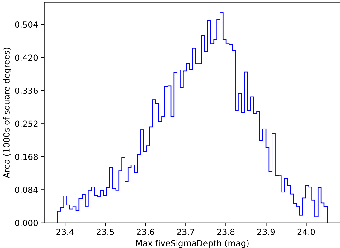
roll_pause_mjdp365_v3.4_10yrs WFD u band: Max fiveSigmaDepth
