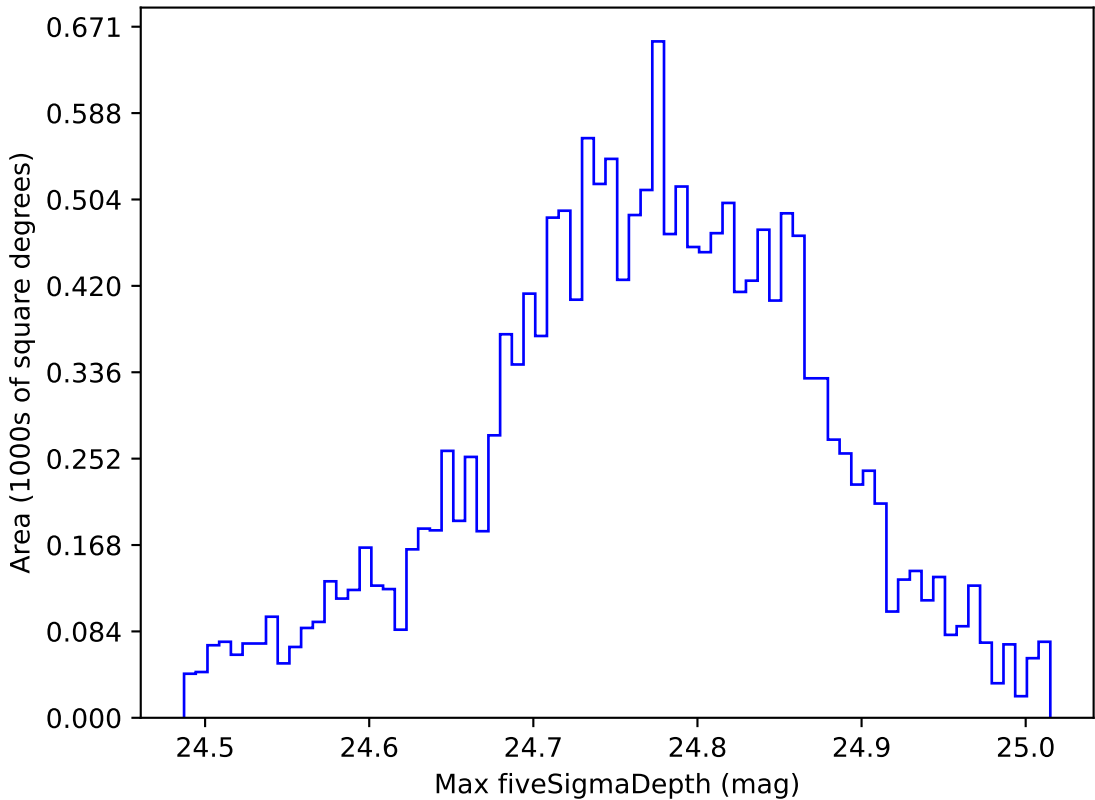
roll_pause_mjdp365_v3.4_10yrs WFD r band: Max fiveSigmaDepth
