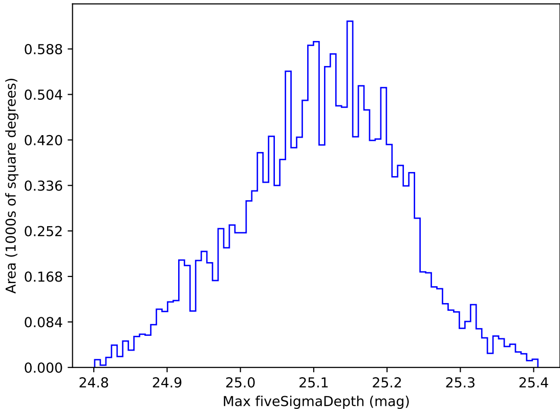
roll_pause_mjdp365_v3.4_10yrs WFD g band: Max fiveSigmaDepth
