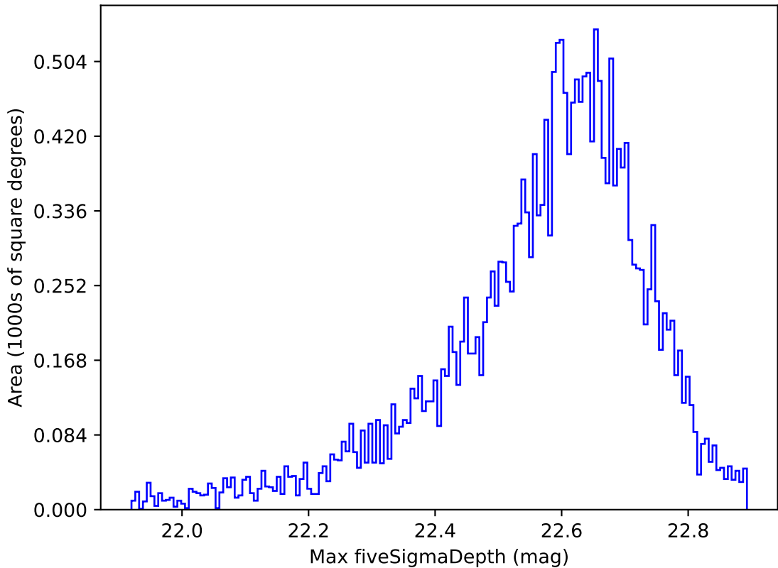
roll_pause_mjdp365_v3.4_10yrs All sky y band: Max fiveSigmaDepth
