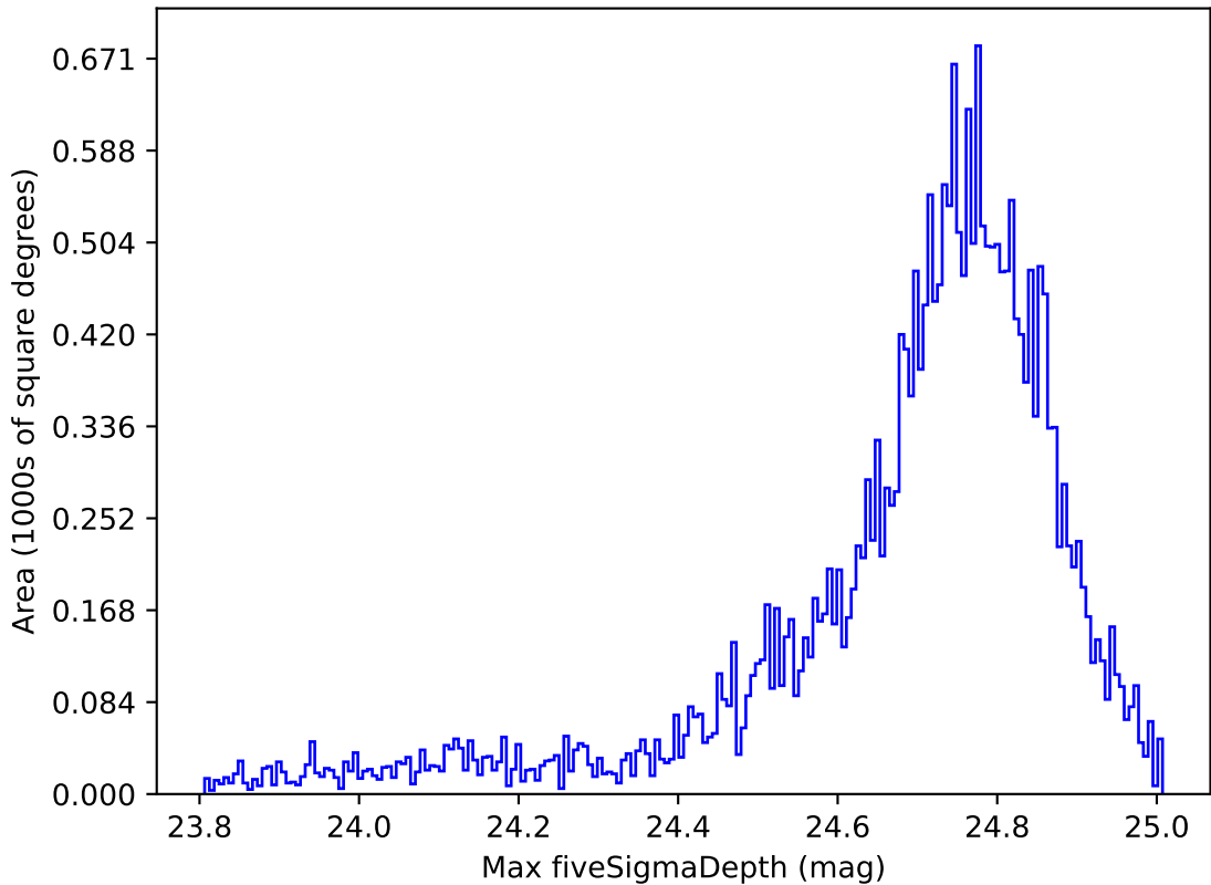
roll_pause_mjdp365_v3.4_10yrs All sky r band: Max fiveSigmaDepth
