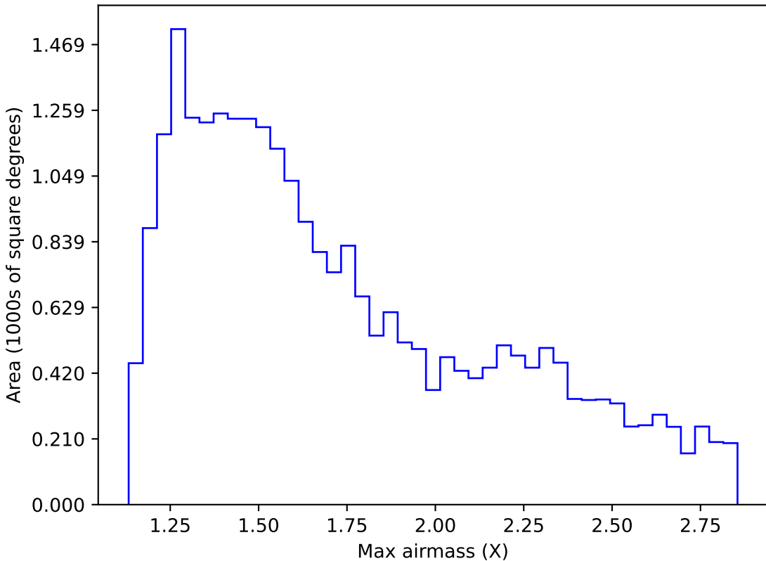
roll_pause_mjdp365_v3.4_10yrs Yr 1 z band: Max airmass
