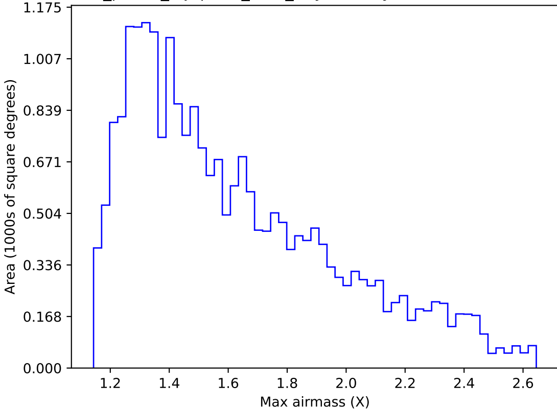
roll_pause_mjdp365_v3.4_10yrs Yr 1 y band: Max airmass
