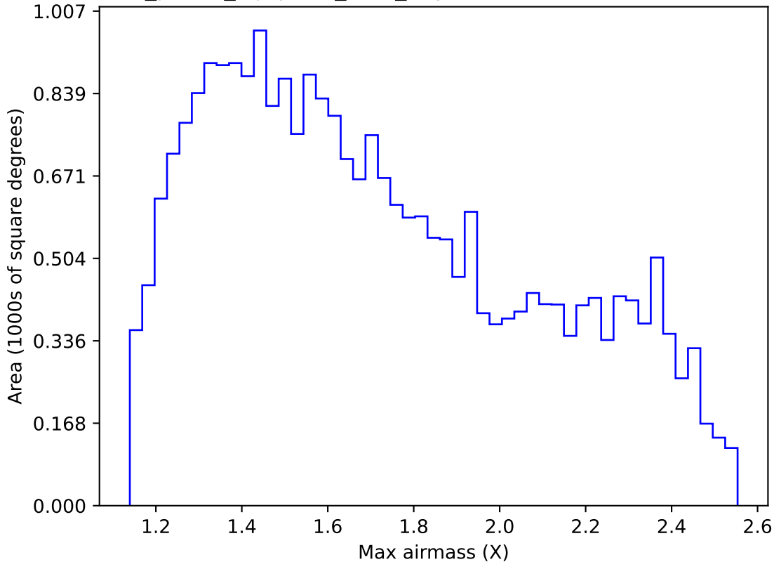
roll_pause_mjdp365_v3.4_10yrs Yr 1 r band: Max airmass
