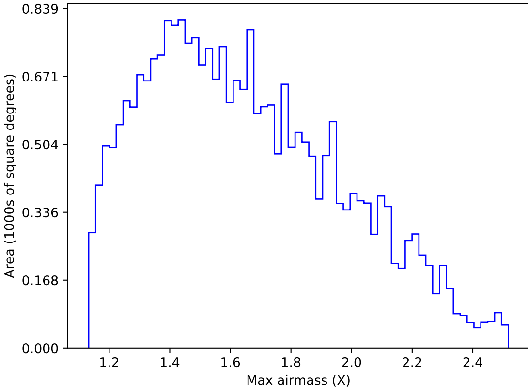
roll_pause_mjdp365_v3.4_10yrs Yr 1 g band: Max airmass
