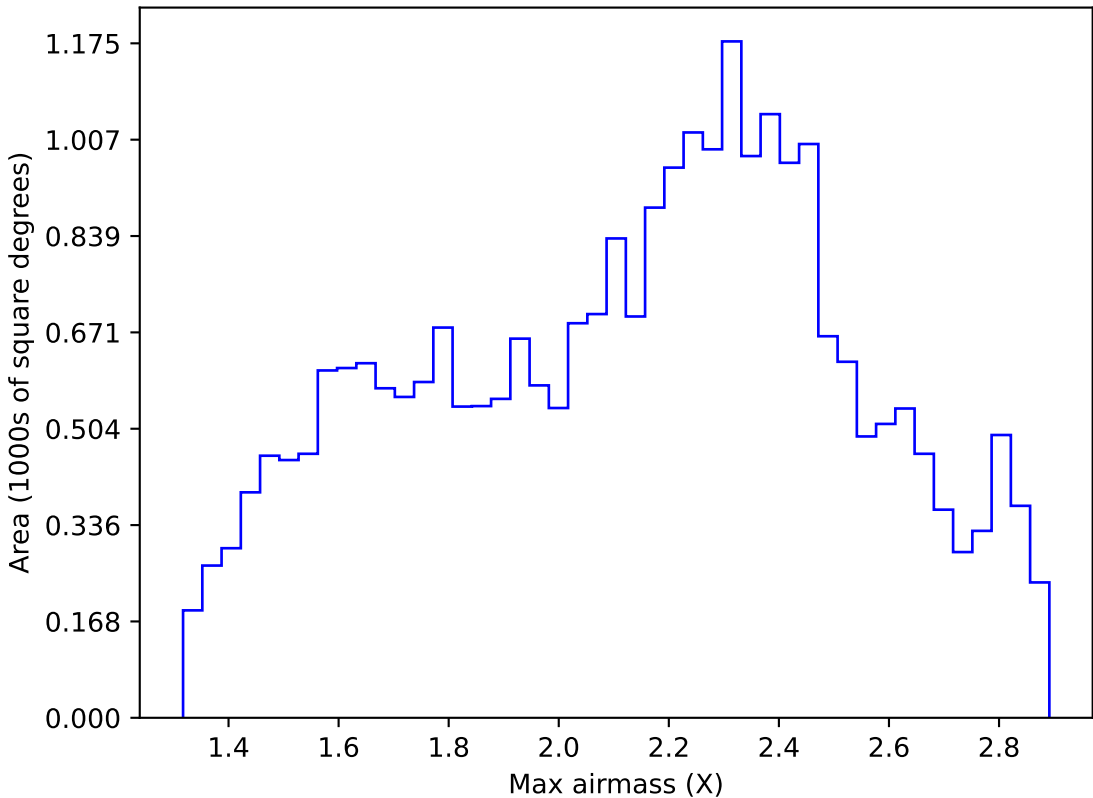
roll_pause_mjdp365_v3.4_10yrs Yr 1 all bands: Max airmass
