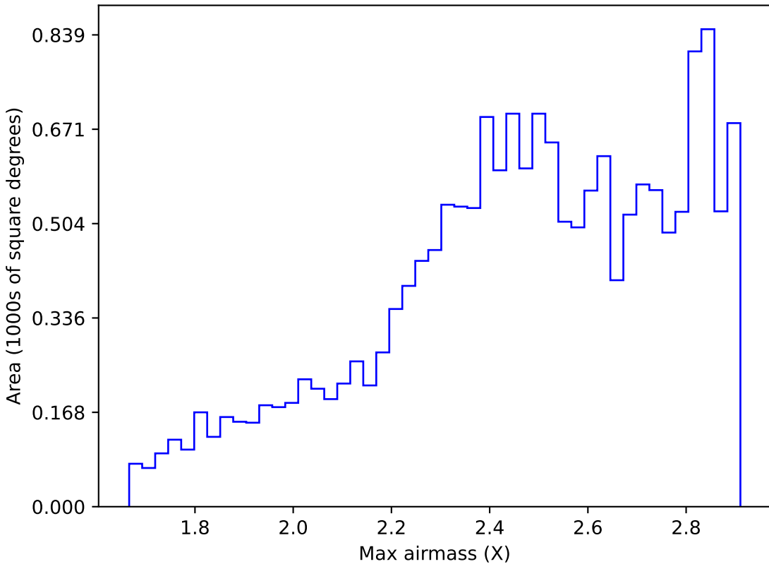
roll_pause_mjdp365_v3.4_10yrs WFD z band: Max airmass
