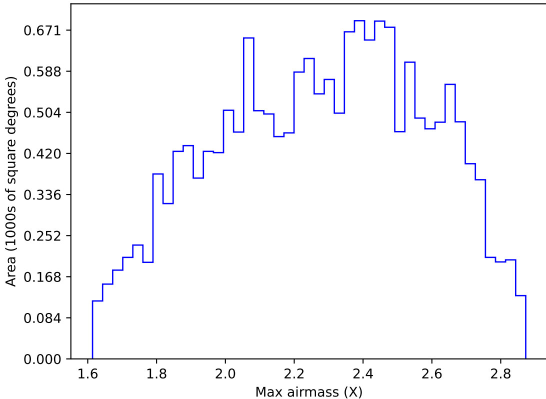
roll_pause_mjdp365_v3.4_10yrs WFD y band: Max airmass
