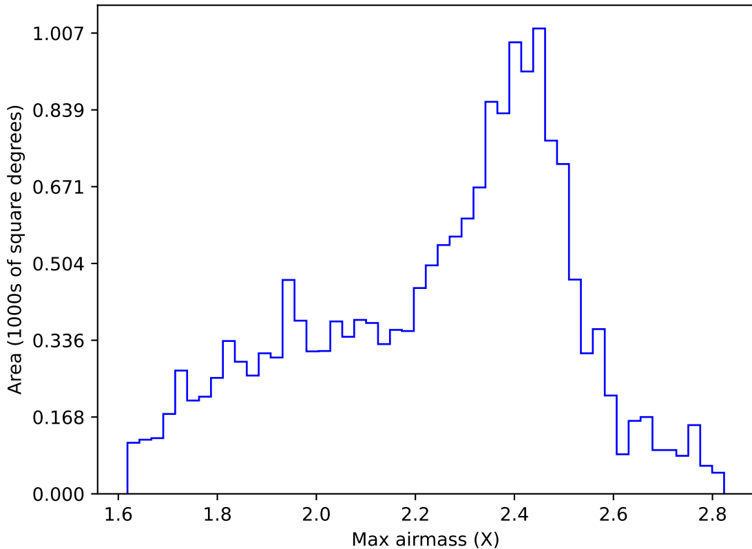
roll_pause_mjdp365_v3.4_10yrs WFD r band: Max airmass
