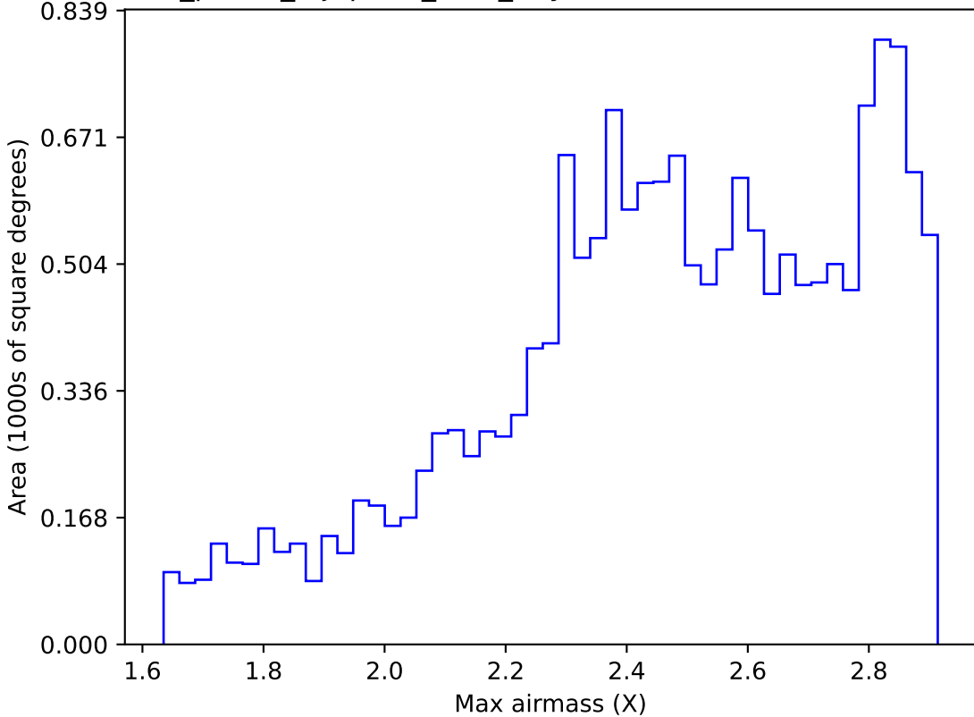
roll_pause_mjdp365_v3.4_10yrs WFD i band: Max airmass
