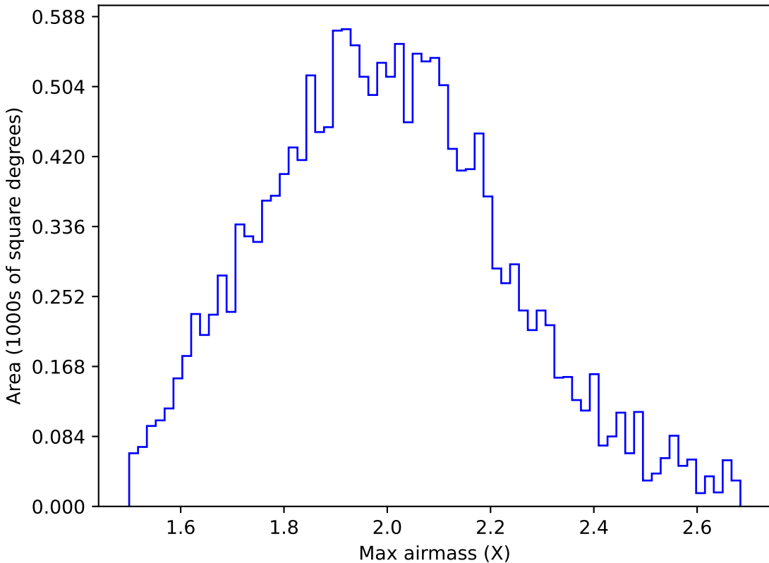
roll_pause_mjdp365_v3.4_10yrs WFD g band: Max airmass
