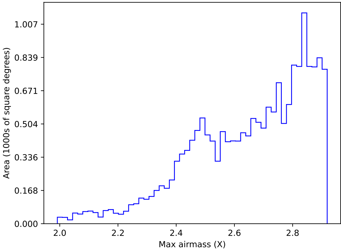
roll_pause_mjdp365_v3.4_10yrs WFD all bands: Max airmass
