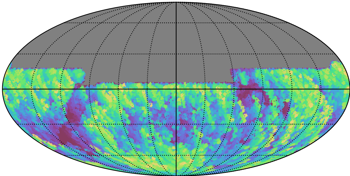
roll_pause_mjdp365_v3.4_10yrs All sky y band: Max airmass
