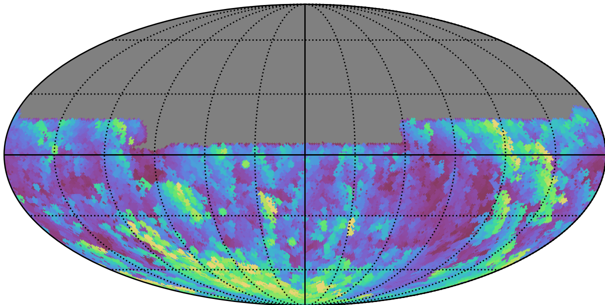
roll_pause_mjdp365_v3.4_10yrs All sky u band: Max airmass
