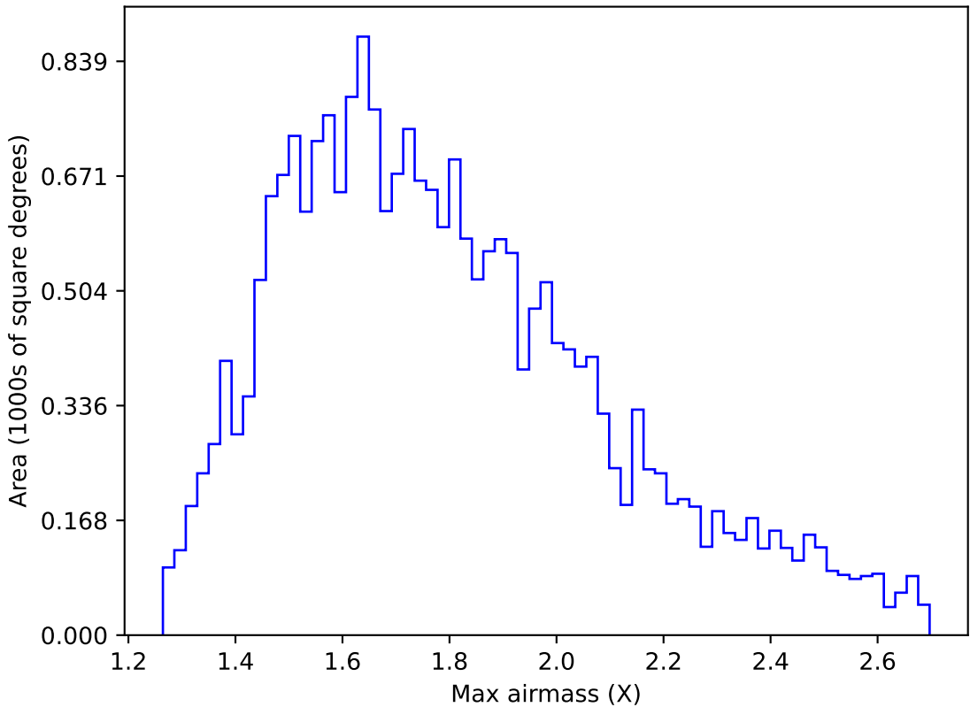
roll_pause_mjdp365_v3.4_10yrs All sky u band: Max airmass
