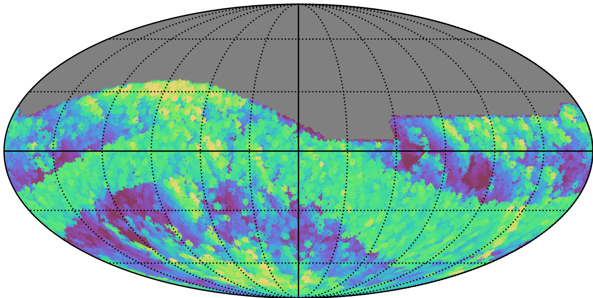
roll_pause_mjdp365_v3.4_10yrs All sky r band: Max airmass
