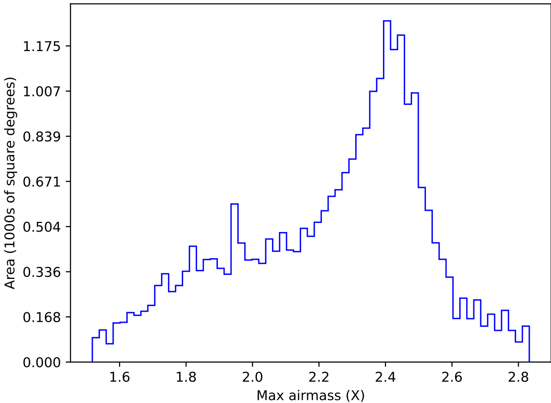
roll_pause_mjdp365_v3.4_10yrs All sky r band: Max airmass
