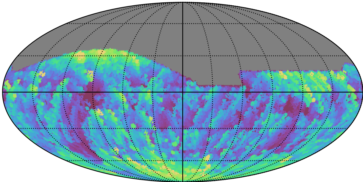
roll_pause_mjdp365_v3.4_10yrs All sky g band: Max airmass
