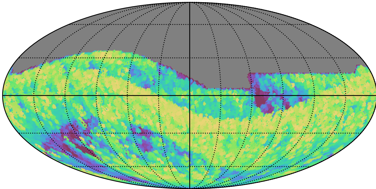
roll_pause_mjdp365_v3.4_10yrs All sky all bands: Max airmass
