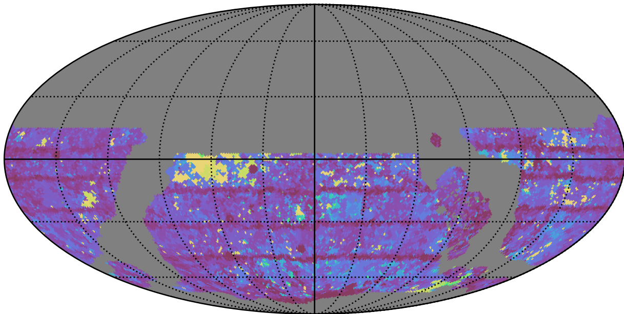
roll_pause_mjdp365_v3.4_10yrs WFD y band: Max Inter-Night Gap
