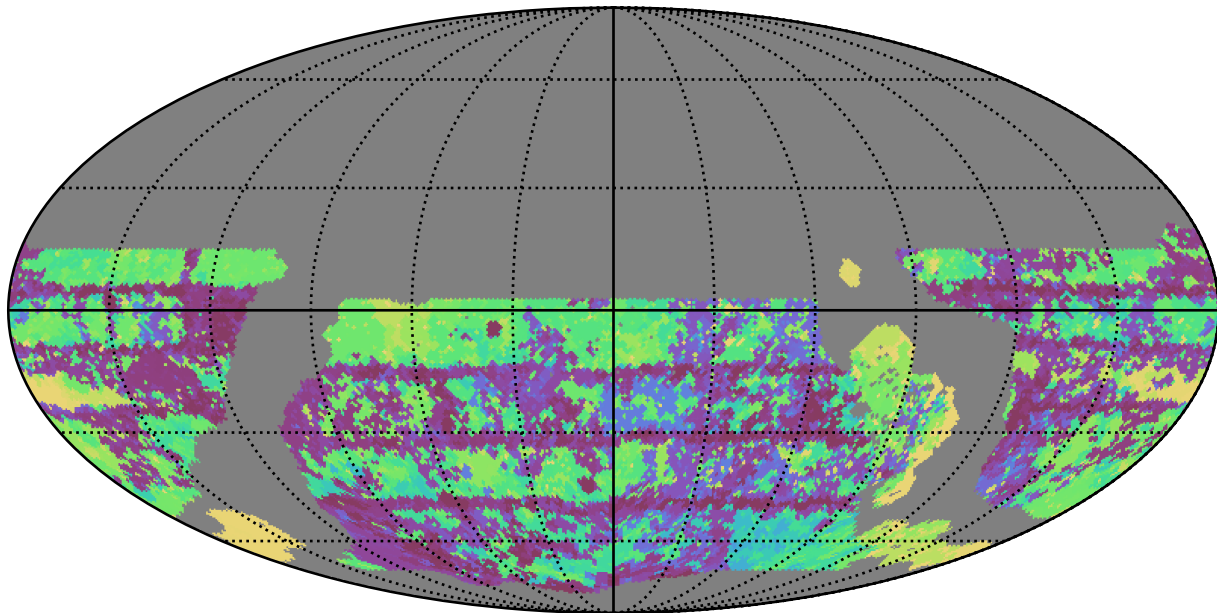
roll_pause_mjdp365_v3.4_10yrs WFD u band: Max Inter-Night Gap
