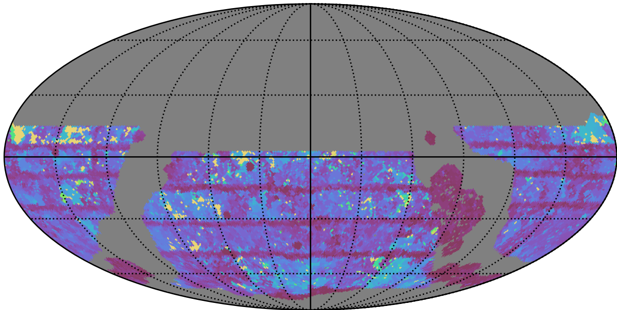
roll_pause_mjdp365_v3.4_10yrs WFD i band: Max Inter-Night Gap
