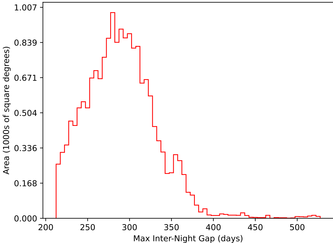
roll_pause_mjdp365_v3.4_10yrs WFD i band: Max Inter-Night Gap
