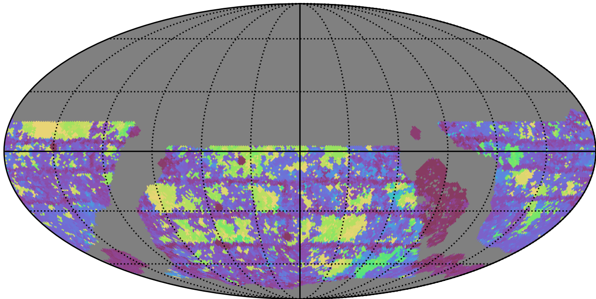
roll_pause_mjdp365_v3.4_10yrs WFD g band: Max Inter-Night Gap
