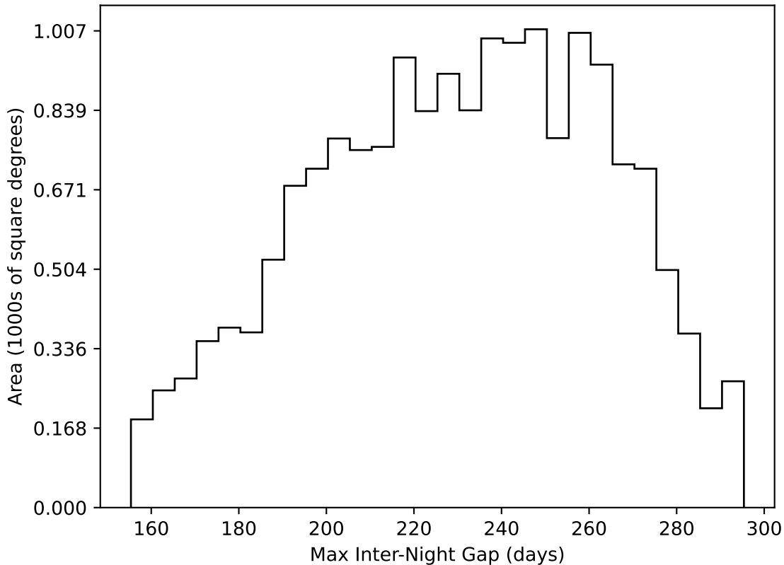
roll_pause_mjdp365_v3.4_10yrs WFD all bands: Max Inter-Night Gap
