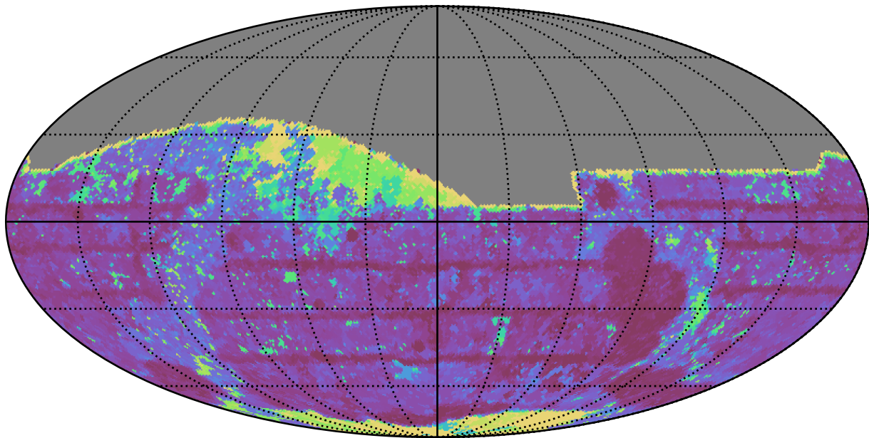
roll_pause_mjdp365_v3.4_10yrs All sky z band: Max Inter-Night Gap
