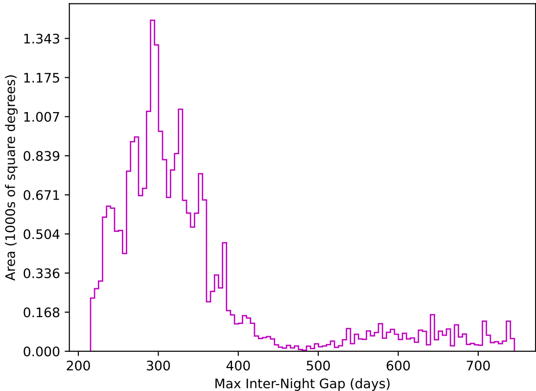
roll_pause_mjdp365_v3.4_10yrs All sky z band: Max Inter-Night Gap
