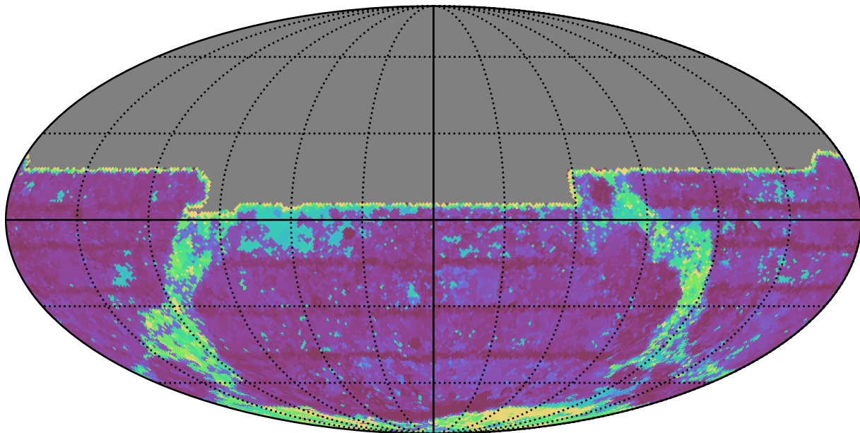
roll_pause_mjdp365_v3.4_10yrs All sky y band: Max Inter-Night Gap
