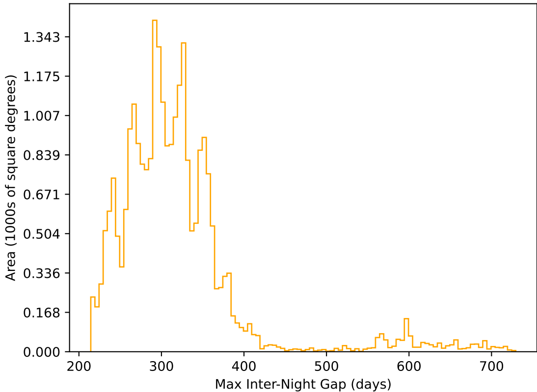
roll_pause_mjdp365_v3.4_10yrs All sky r band: Max Inter-Night Gap
