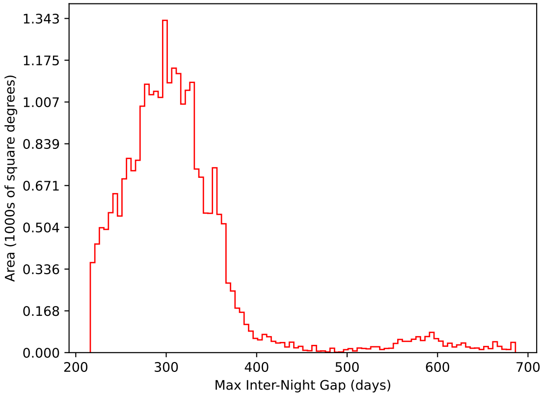
roll_pause_mjdp365_v3.4_10yrs All sky i band: Max Inter-Night Gap
