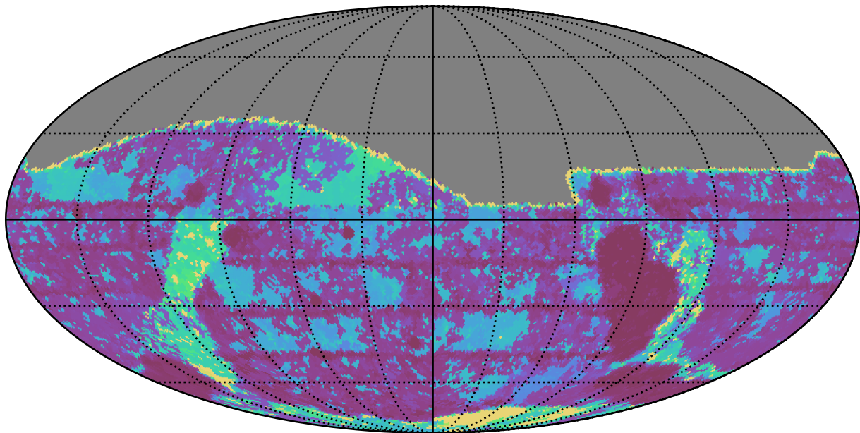
roll_pause_mjdp365_v3.4_10yrs All sky g band: Max Inter-Night Gap
