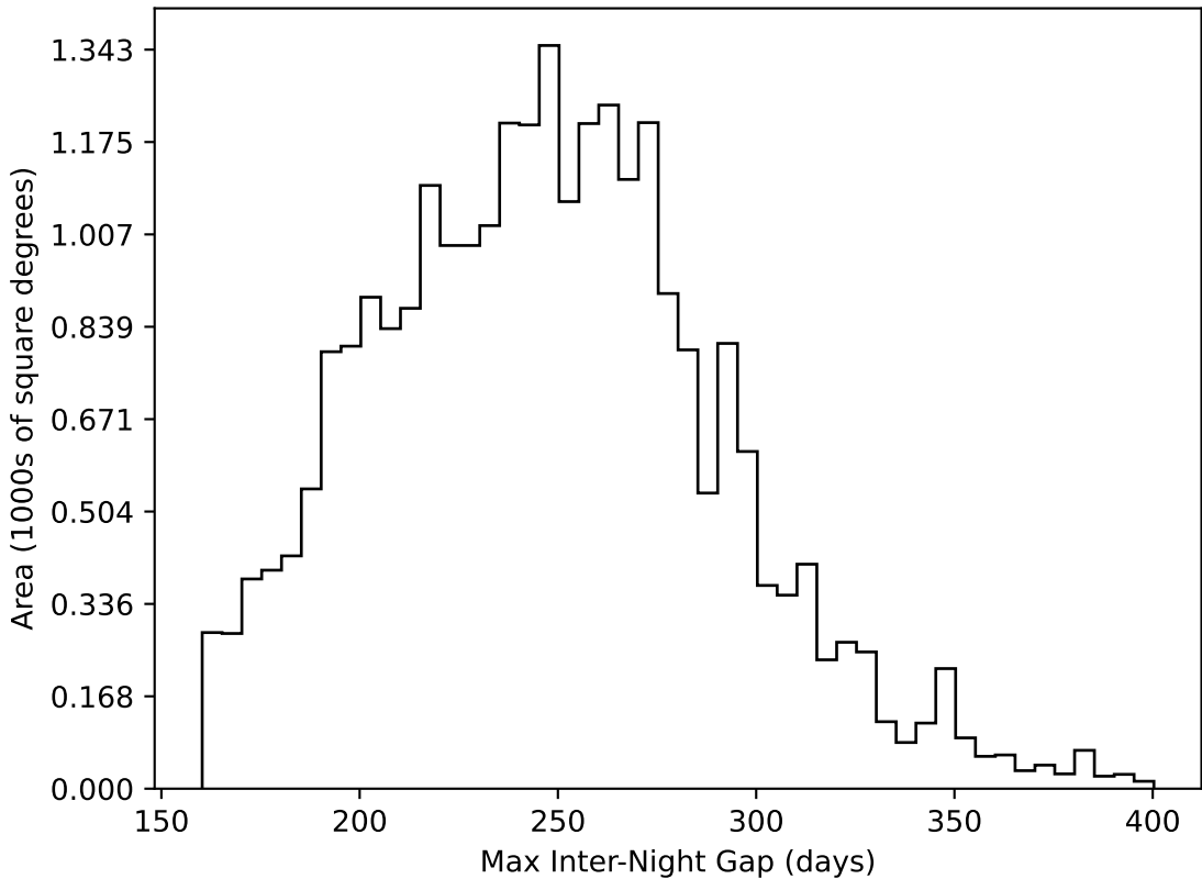
roll_pause_mjdp365_v3.4_10yrs All sky all bands: Max Inter-Night Gap
