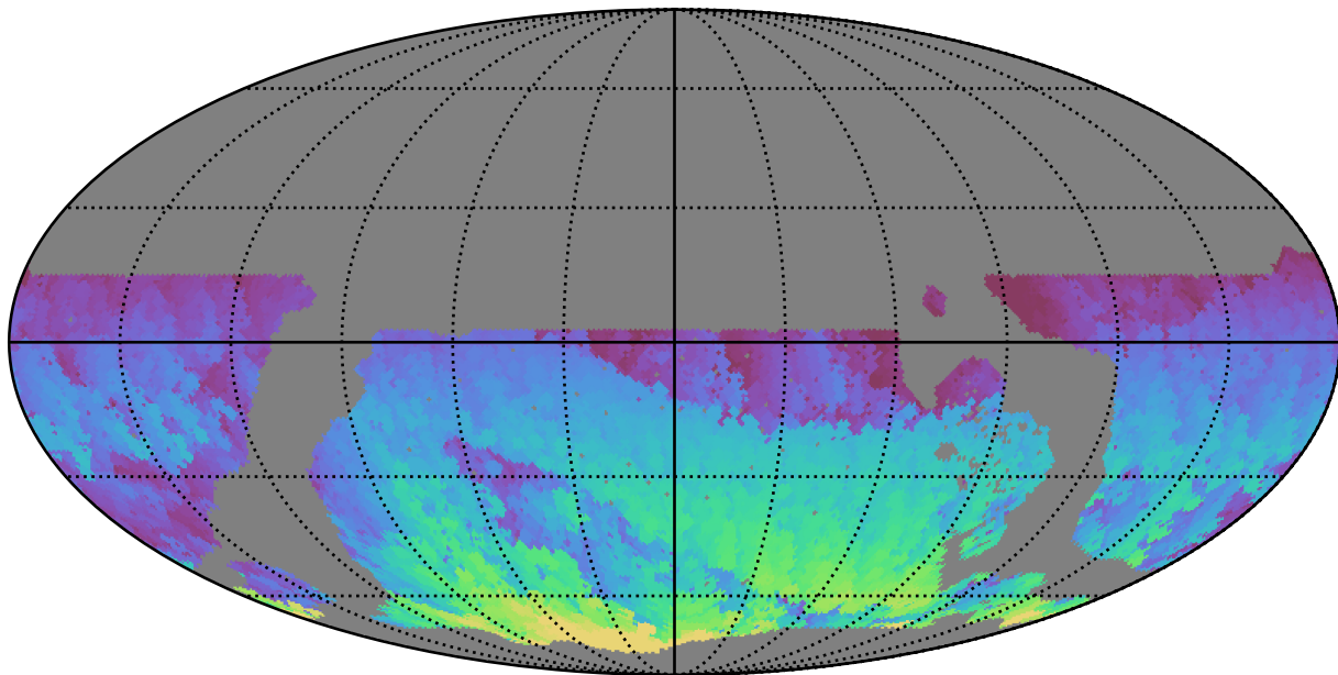
roll_pause_mjdp365_v3.4_10yrs WFD z band: Max HA
