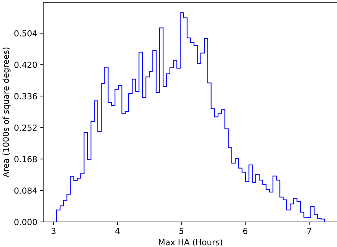
roll_pause_mjdp365_v3.4_10yrs WFD z band: Max HA
