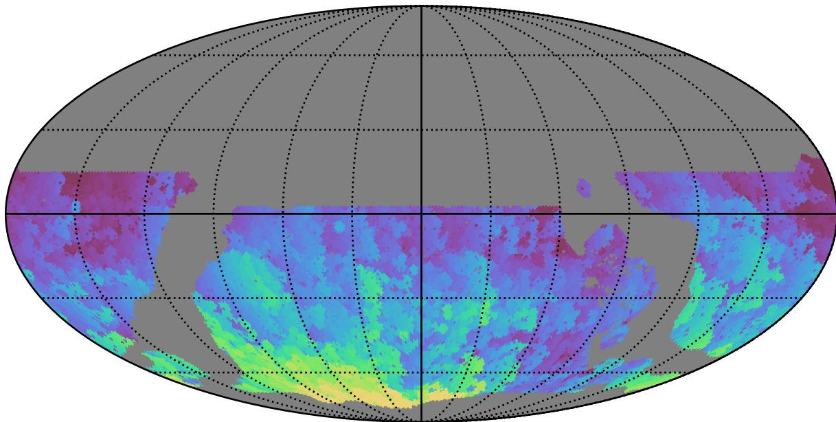
roll_pause_mjdp365_v3.4_10yrs WFD u band: Max HA
