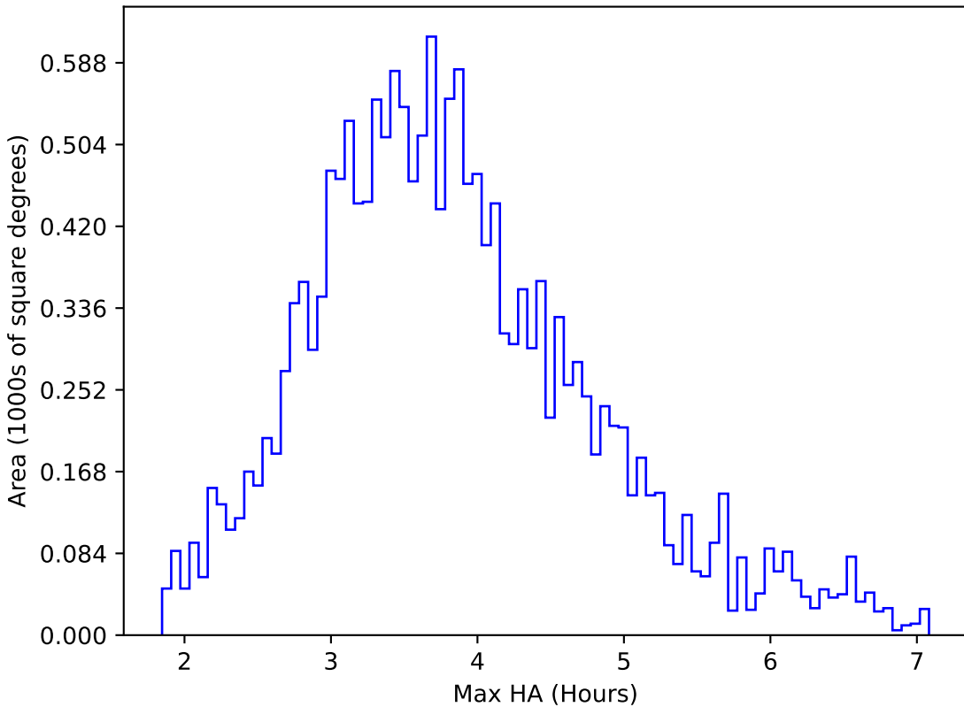
roll_pause_mjdp365_v3.4_10yrs WFD u band: Max HA
