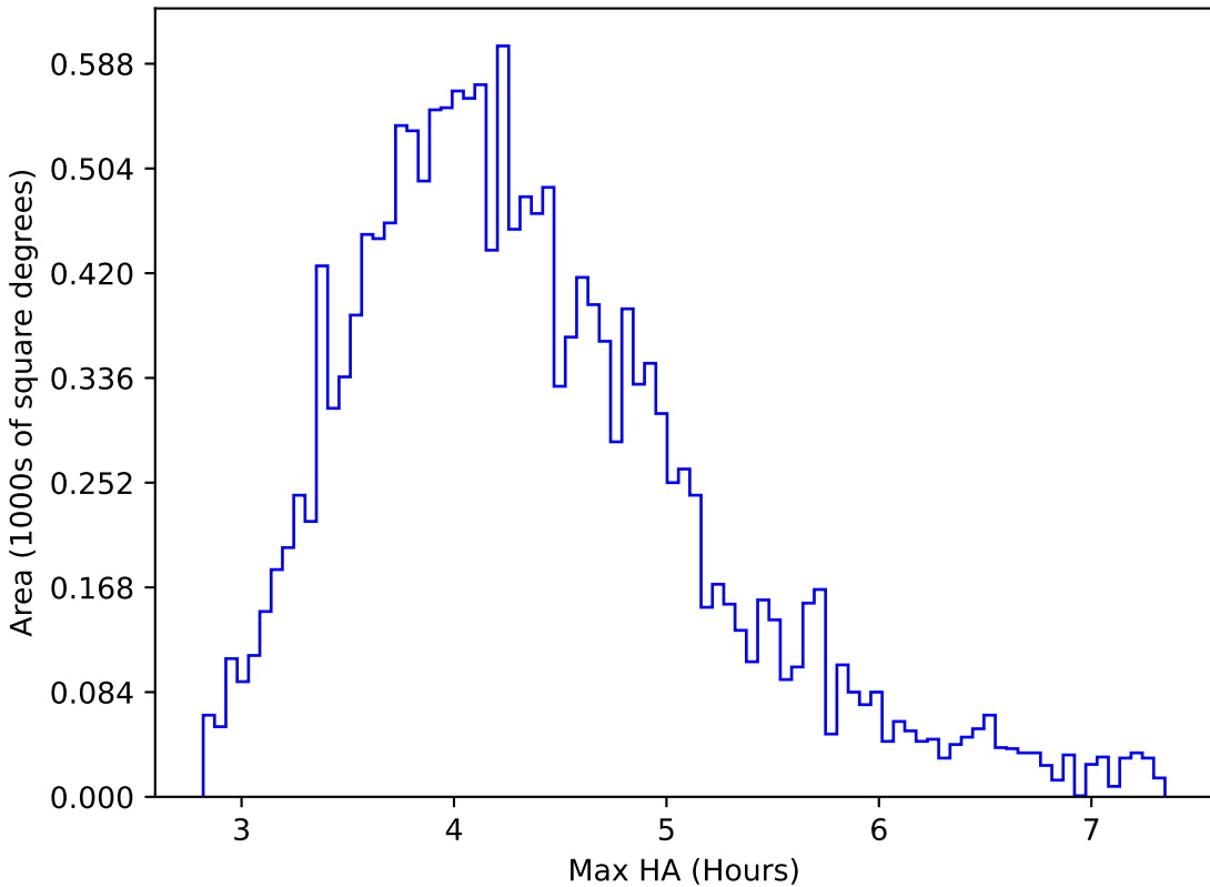
roll_pause_mjdp365_v3.4_10yrs WFD r band: Max HA
