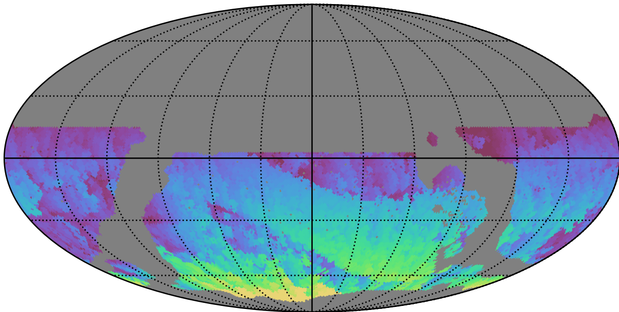
roll_pause_mjdp365_v3.4_10yrs WFD i band: Max HA
