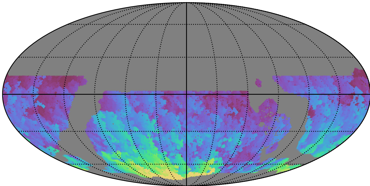
roll_pause_mjdp365_v3.4_10yrs WFD g band: Max HA
