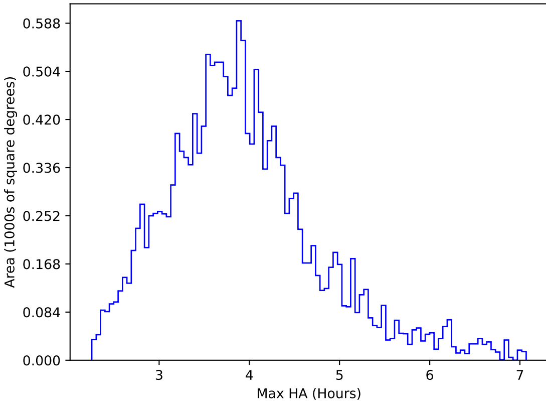
roll_pause_mjdp365_v3.4_10yrs WFD g band: Max HA
