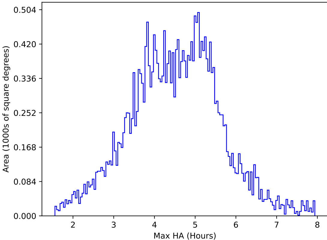
roll_pause_mjdp365_v3.4_10yrs All sky z band: Max HA
