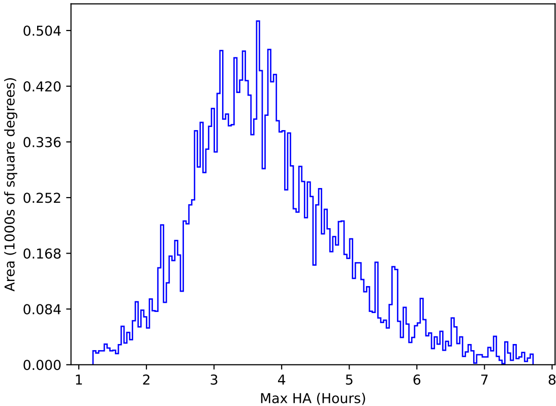
roll_pause_mjdp365_v3.4_10yrs All sky u band: Max HA
