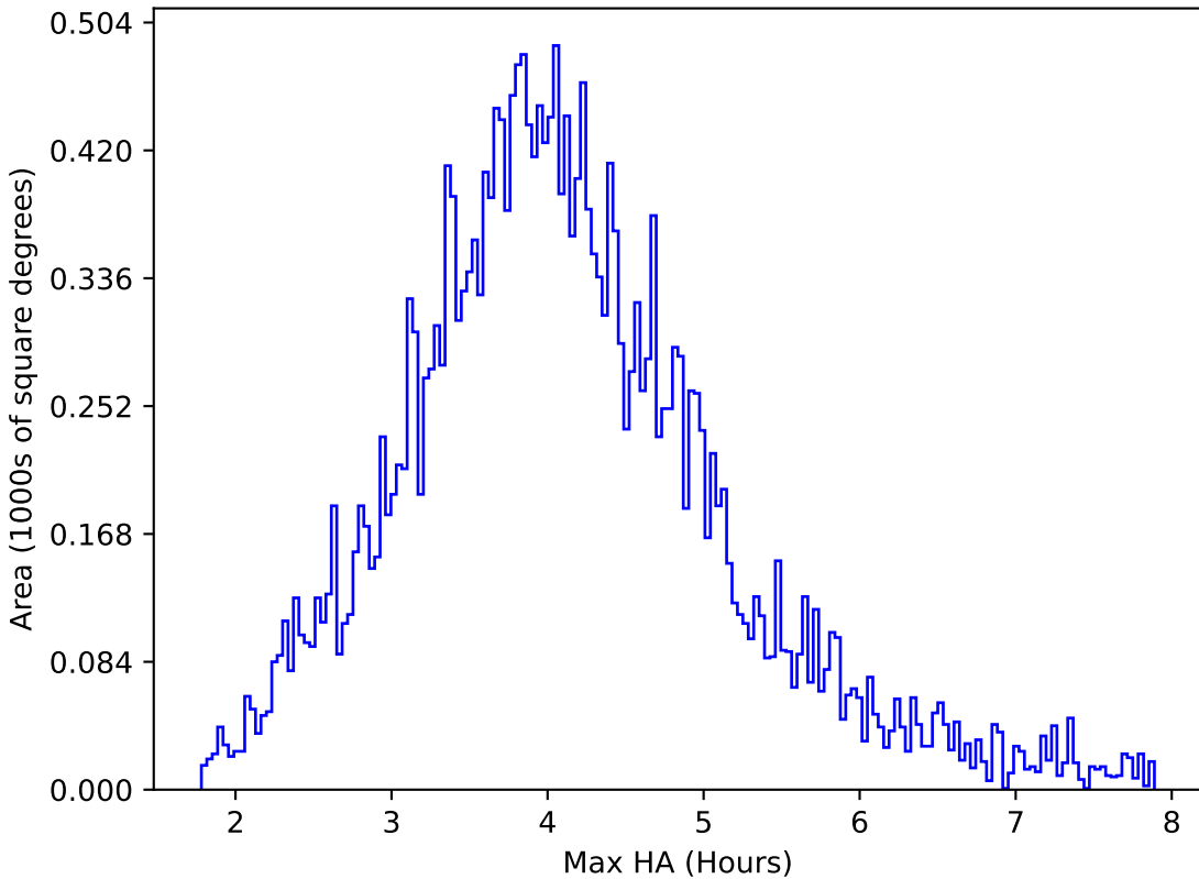
roll_pause_mjdp365_v3.4_10yrs All sky r band: Max HA
