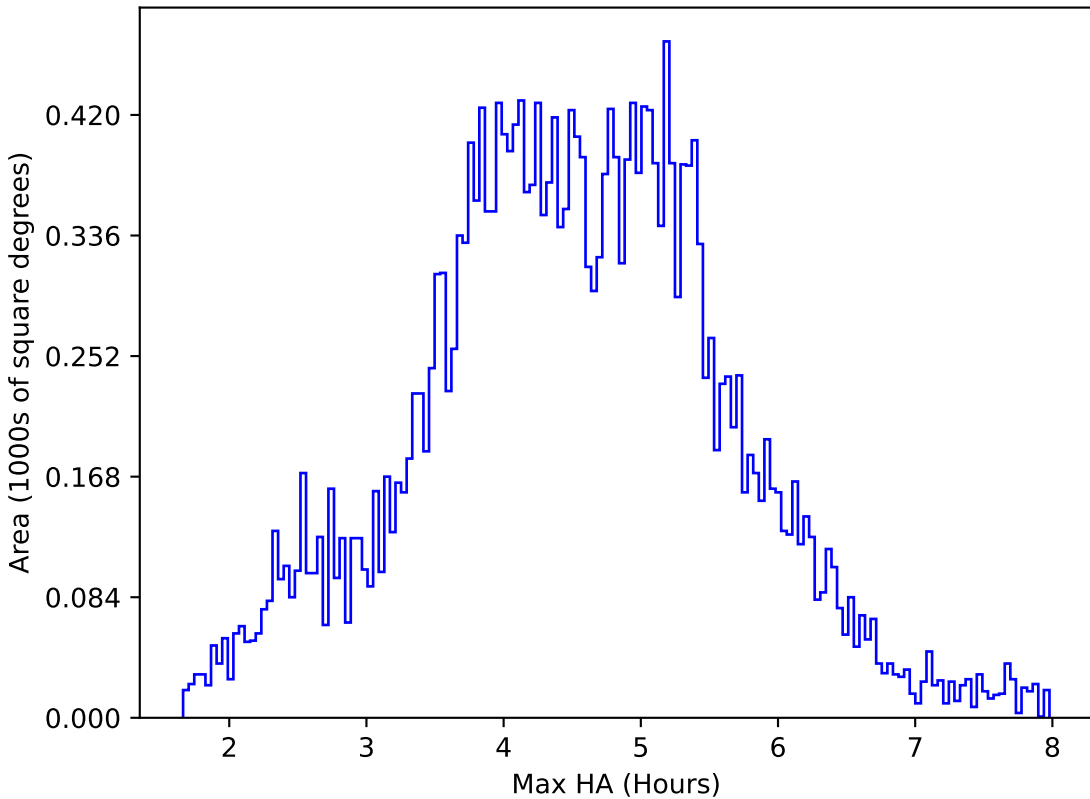
roll_pause_mjdp365_v3.4_10yrs All sky i band: Max HA
